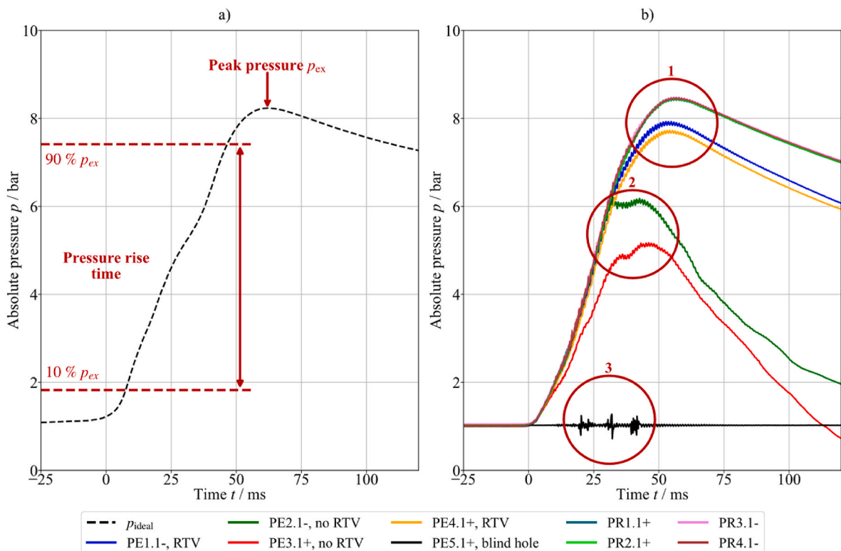
Fig. 4.1. Comparison of the idealized a) and actual time-resolved pressure curve; b) of a \text{C}_3\text{H}_8 -air explosion and TR (P-TR).
